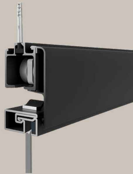
Ceiling mounted sliding rail
