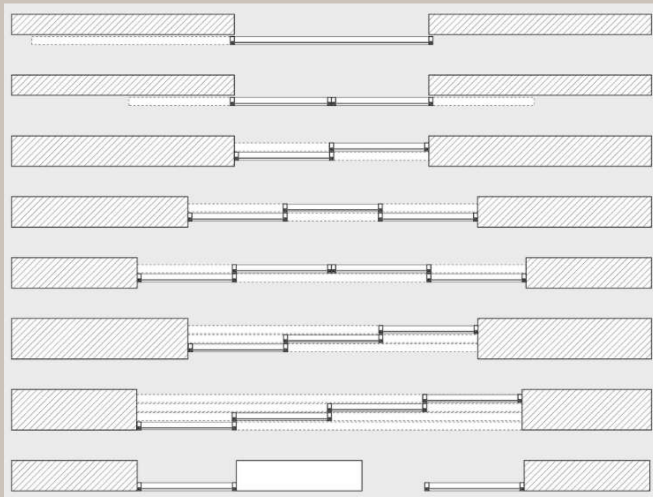
Sliding Doors Track & Pane Options
