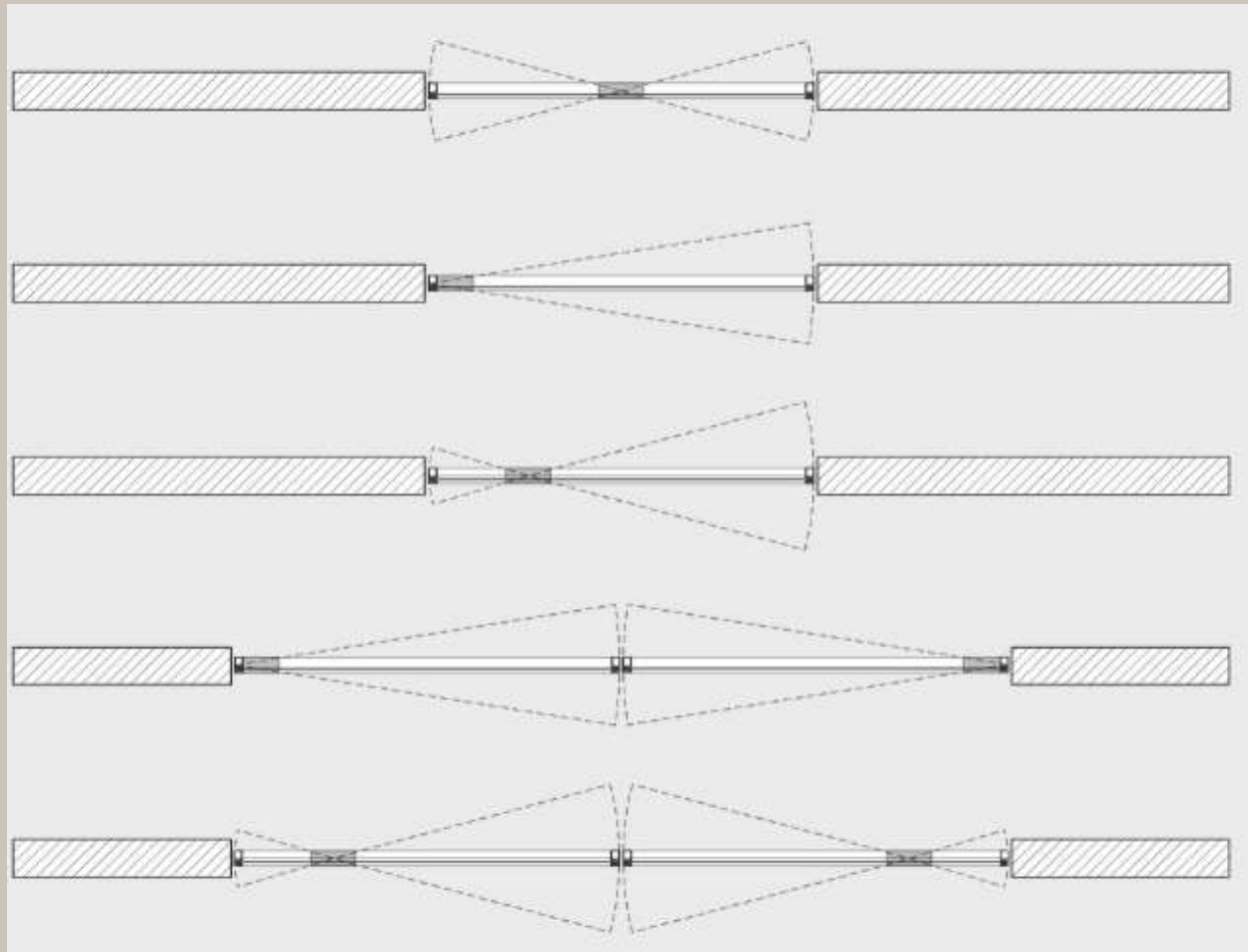
Pivot Doors Opening Options
