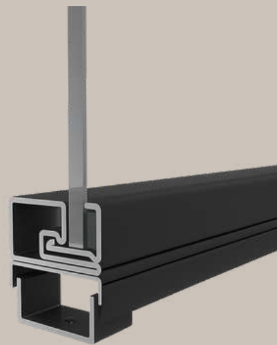
Concealed lower door guide
