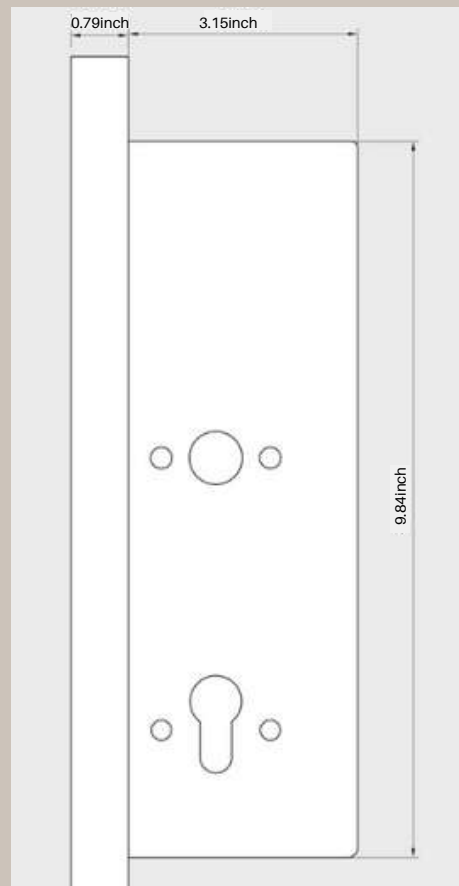
Standard lock-cassette dimensions
